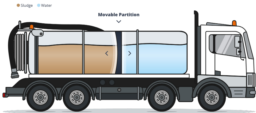
Movable partition. As the water in the tank gets used, the partition moves to give space for the sludge.
