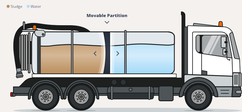
Movable partition. As the water in the tank gets used, the partition moves to give space for the sludge.
